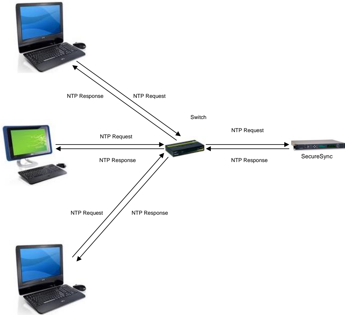
Figure 2: Testing NTP Request Threshold with Multiple Hosts
