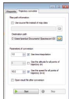
Figure 4: Trajectory Converter
